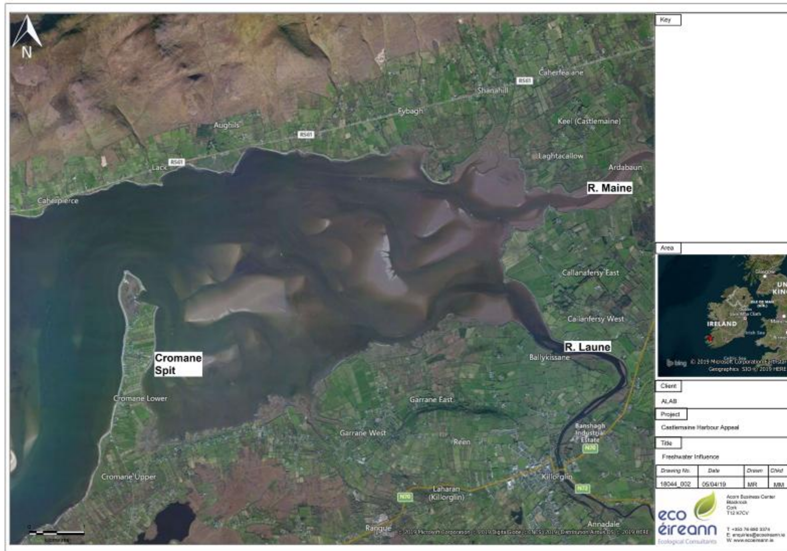
Figure 2 Freshwater Influences
