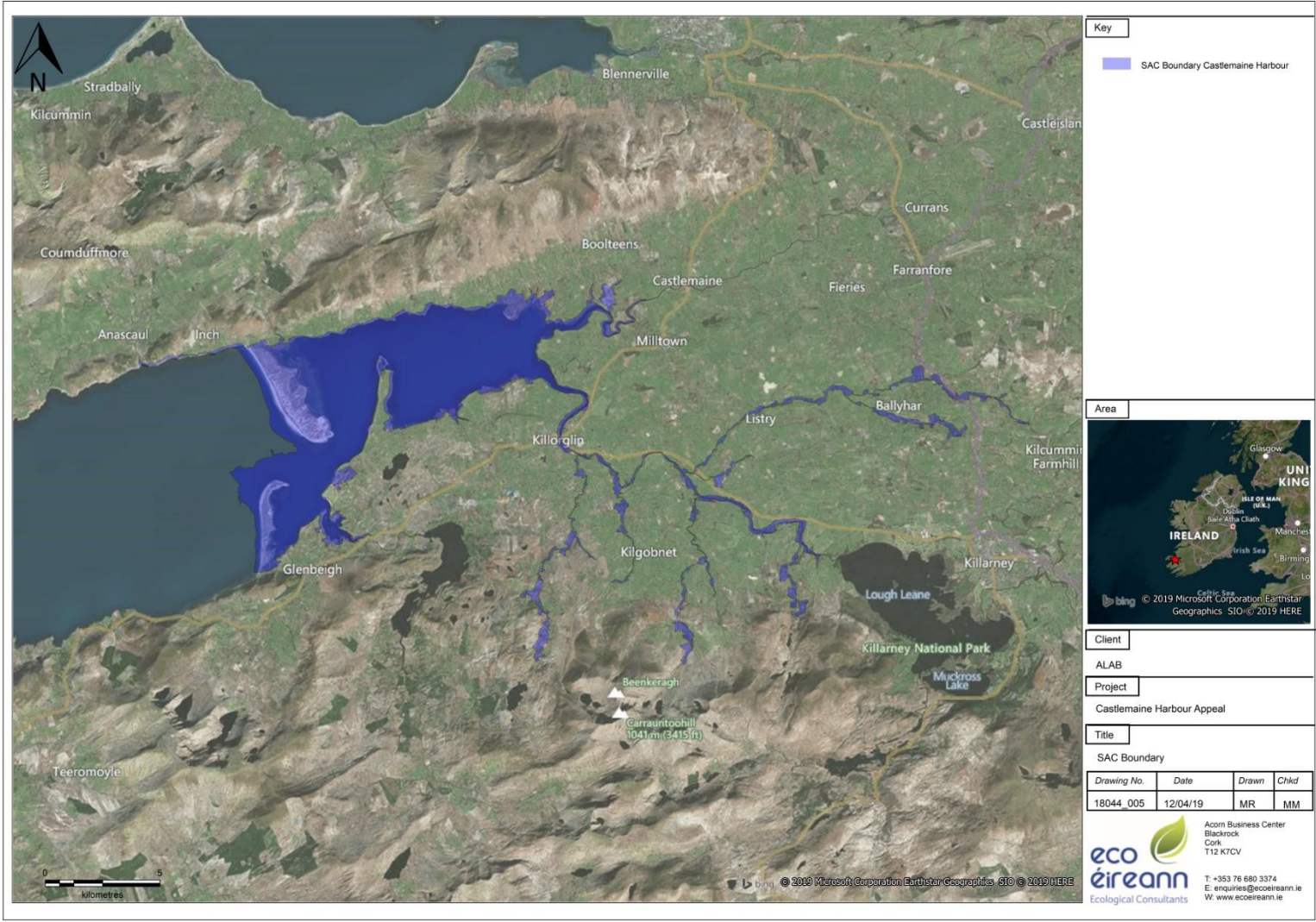
Figure 6 SAC Boundary
