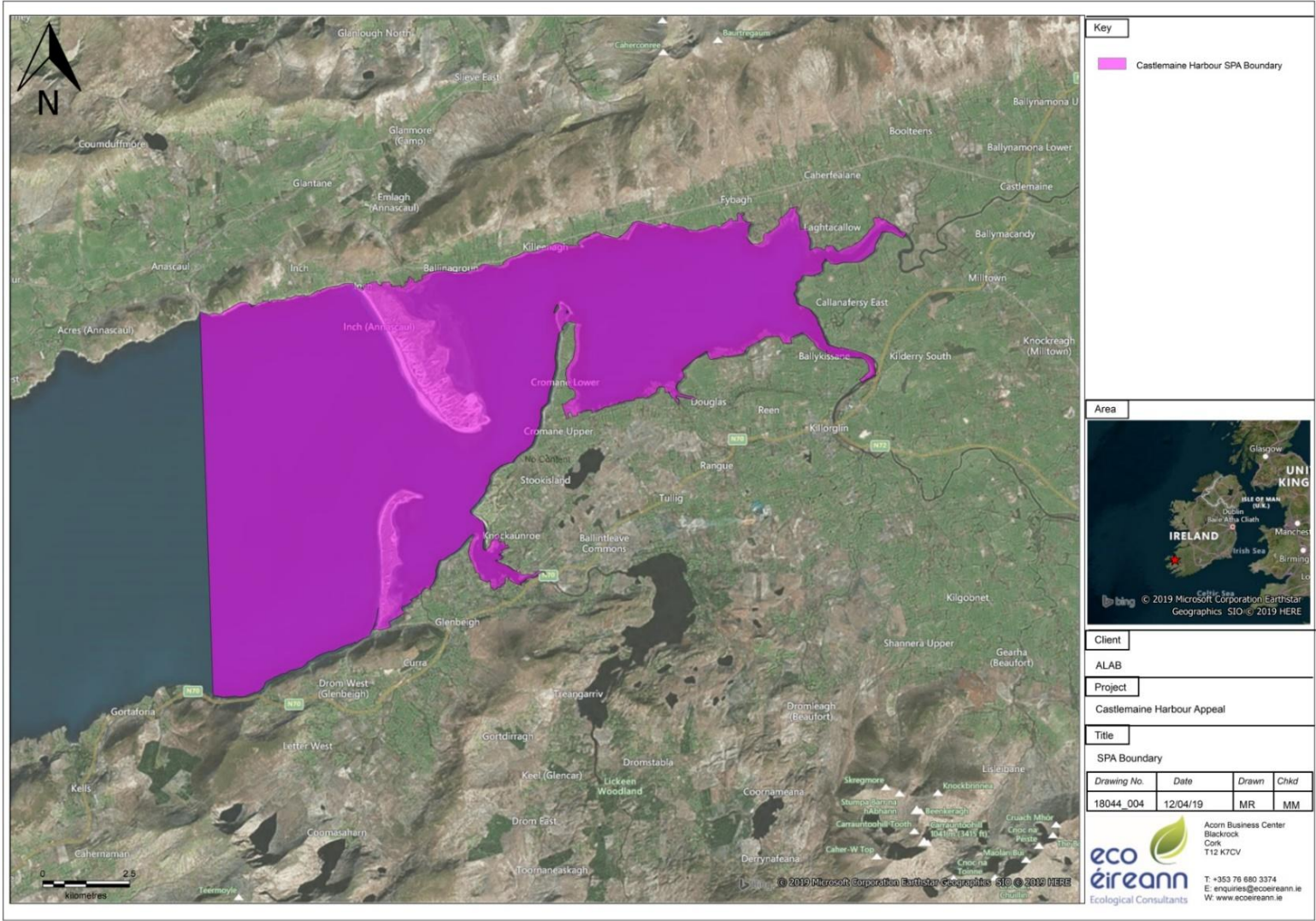
Figure 7 SPA Boundary
